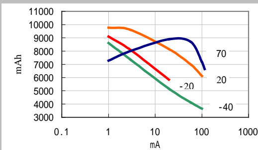
CAPACITY VS. CURRENT
